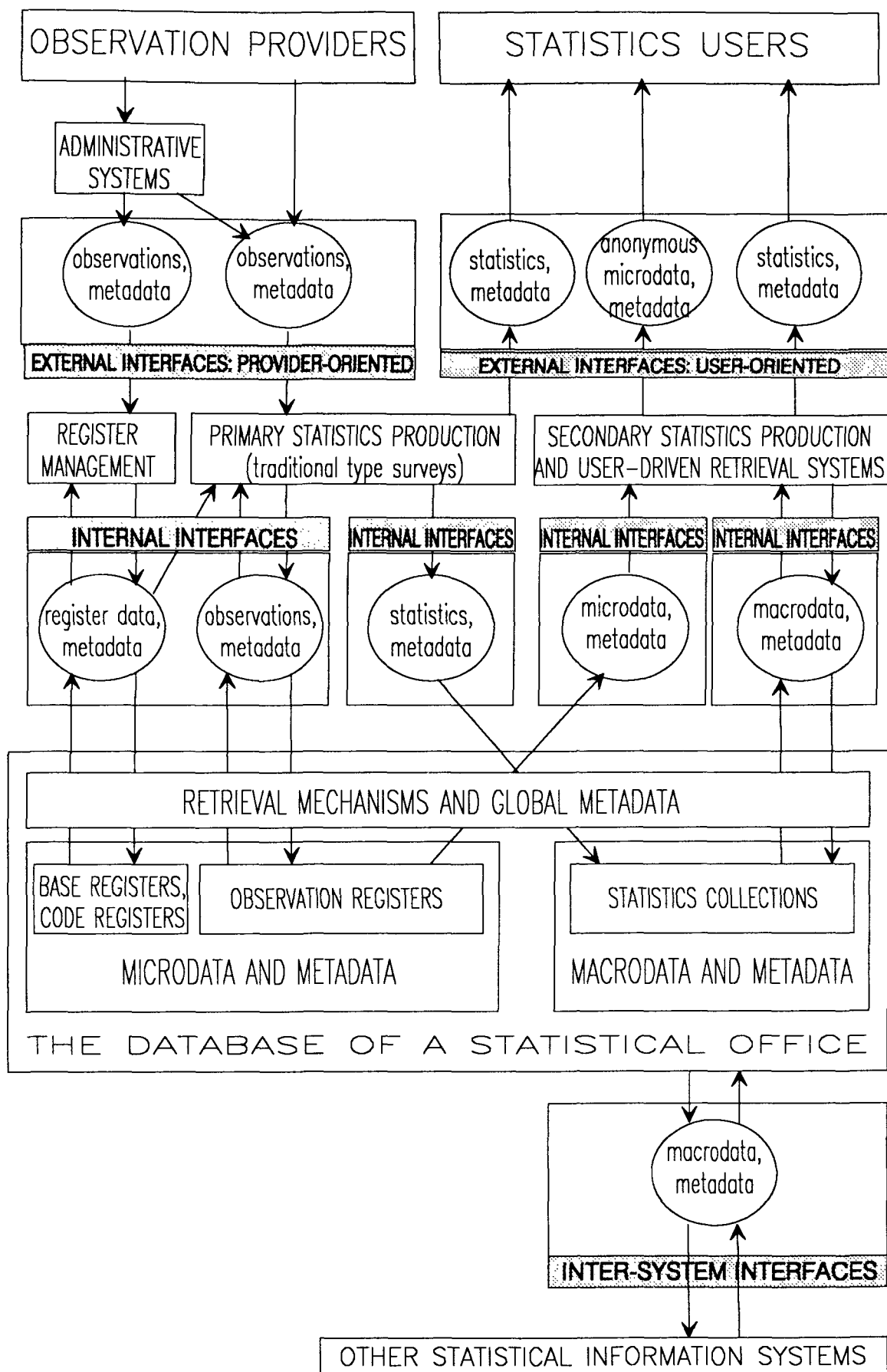
Figure 1.4. A model of a self-describing database-oriented statistical information system.
