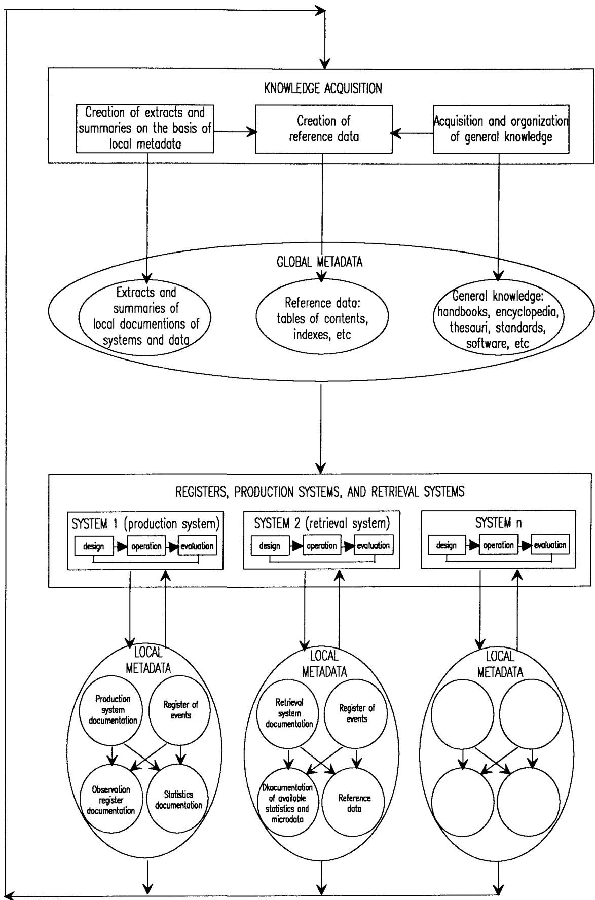
Figure 5.2. Metadata flows for a system of different kinds of statistical information systems.
