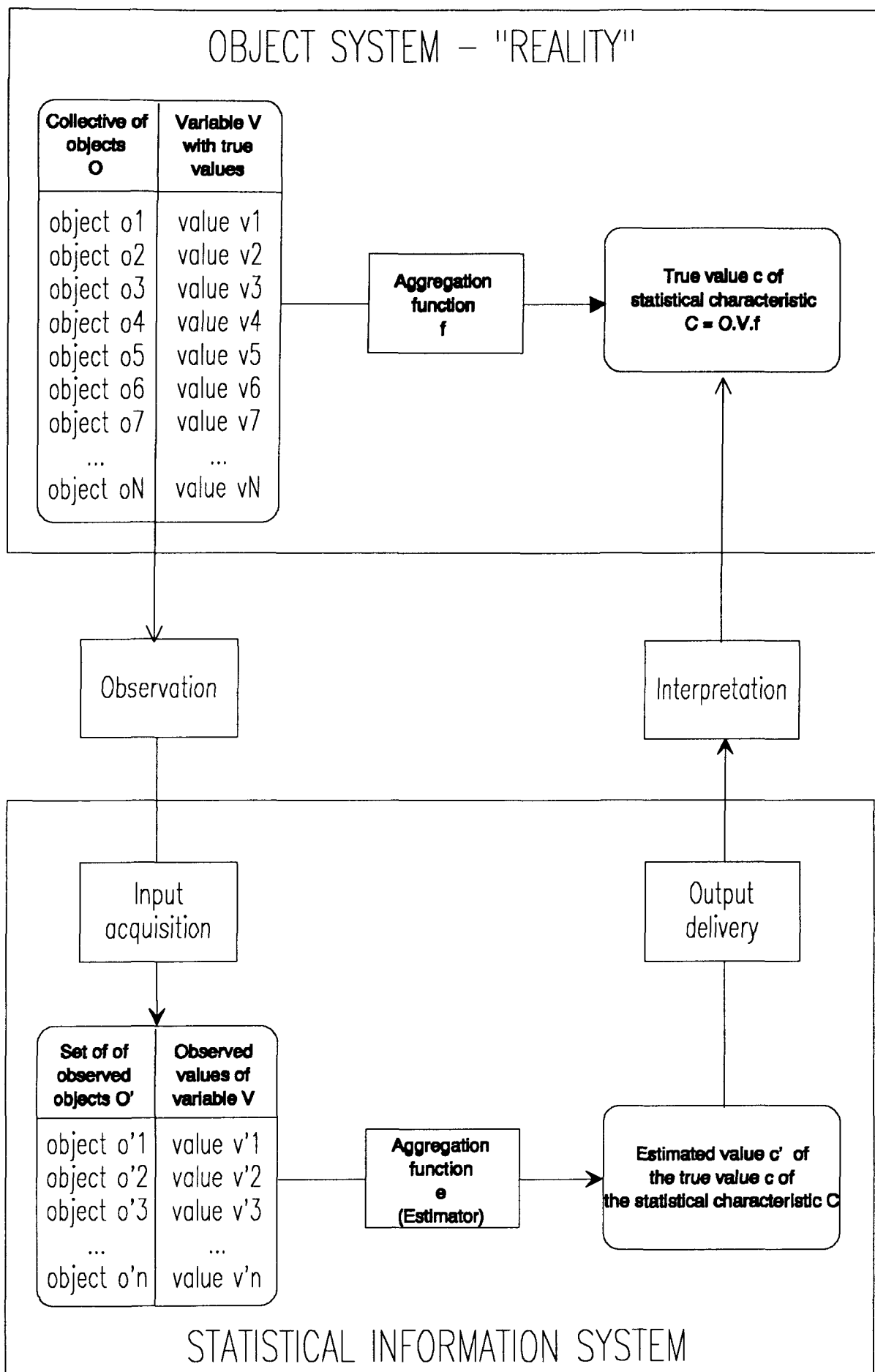
Figure 1.1. Illustration of some fundamental concepts in statistical information processing.
