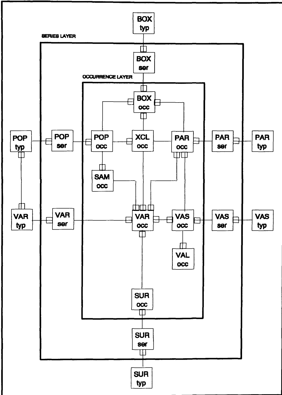
Figure 5.1. A metaobject graph modelling the contents of a statistical metadata database.
