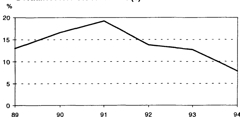
Diagram 2 Bortfallet i KYBOK 1989-1994 (1) 1
