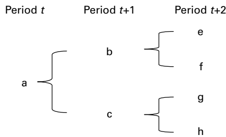
Fig. 1. Growing Family Tree
