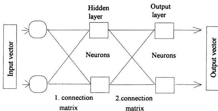
Fig. 3 Two-layer network
